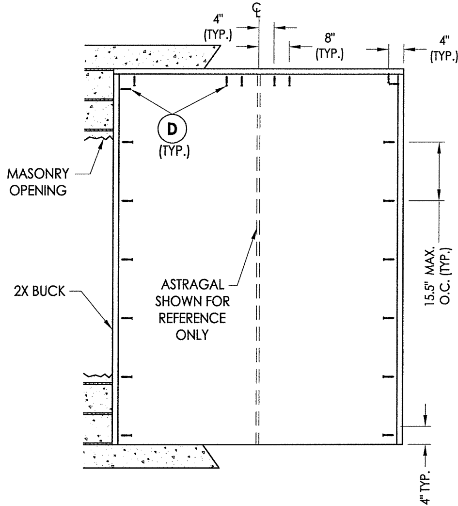
BUCK ANCHORING
