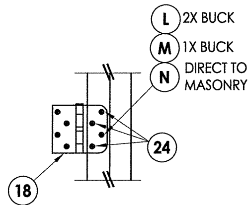
HINGE DETAIL
